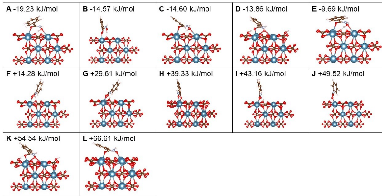
Figure S10. Related to Figure 2 and Table 2: Side views of DFT structures for adsorption of BHA on calcite- [10\bar{1}4] , including acidic hydrogens. For simplicity, only three layers of the surface slab are shown. Color scheme: Ca: dark blue, C: brown, O: red, N: light blue, H: white. Adsorption energies are also given for each structure. Structures result from conformational search described in Transparent Methods section of this file. Species A is that shown in the center panel of Figure 2 of the main text.
