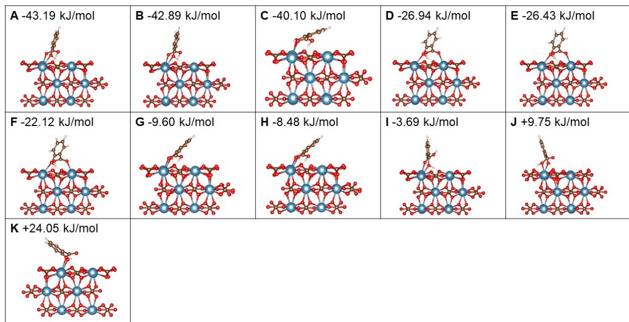
Figure S11. Related to Figure 2 and Table 2: Side views of DFT structures for adsorption of SA on calcite- [10\bar{1}4] , including acidic hydrogens. For simplicity, only three layers of the surface slab are shown. Color scheme: Ca: dark blue, C: brown, O: red, N: light blue, H: white. Adsorption energies are also given for each structure. Structures result from conformational search described in Transparent Methods section of this file. Species A is that shown in the right panel of Figure 2 of the main text.
