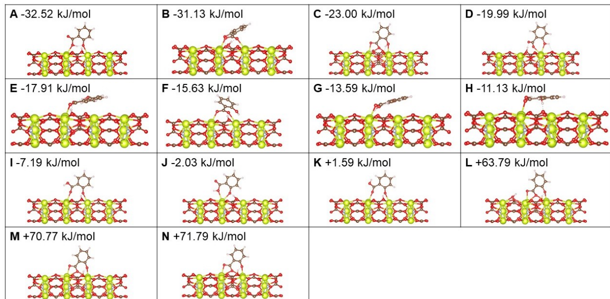
Figure S8. Related to Figure 1 and Table 2: Side views of DFT structures for adsorption of SA on bastnäsite-[10 \bar{1} 0], including acidic hydrogens. For simplicity, only three layers of the surface slab are shown. Color scheme: Ce: green, C: brown, O: red, F/N: light blue, H: white. Adsorption energies are also given for each structure. Structures result from conformational search described in Transparent Methods section of this file. Species A is that shown in the right panel of Figure 1 of the main text.
